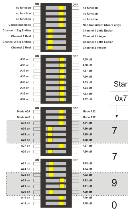
Figure 7 DIP switch, settings for ALSPA C80 HPCi (one, respectively first ibaLink-VME card)
