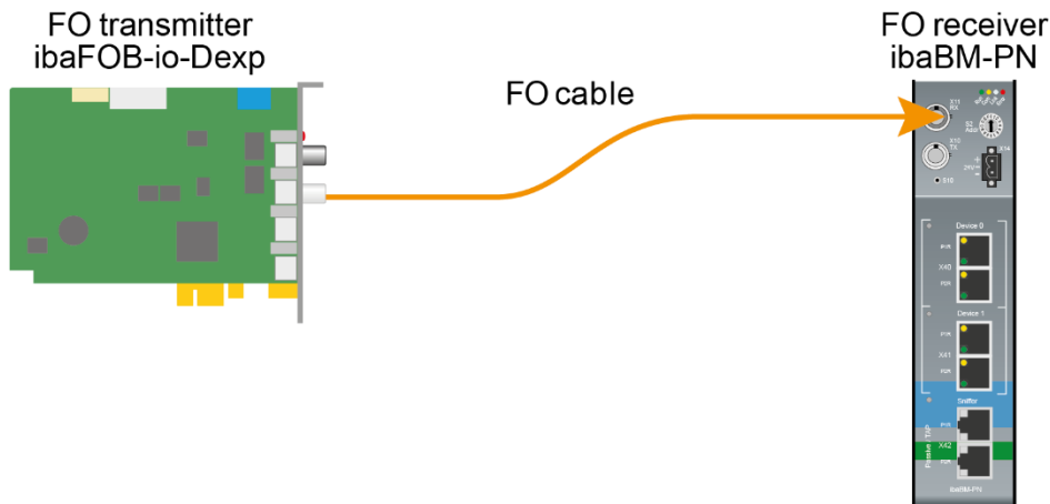
Figure 1: Example: simple connection for FO budget calculation
