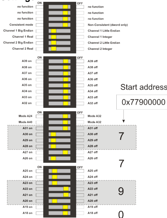
Figure 5 DIP switch, settings for ALSPA C80 HPC (one, respectively first ibaLink-VME card)
